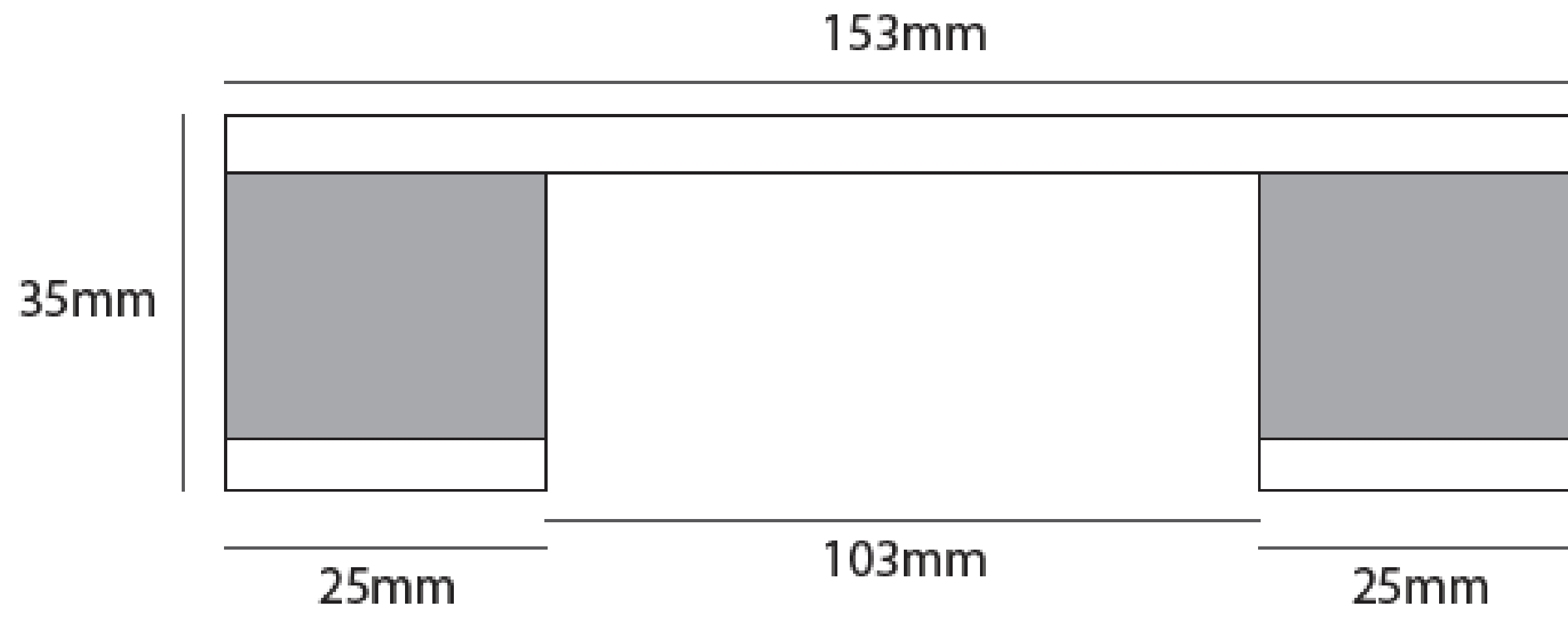
Side view
