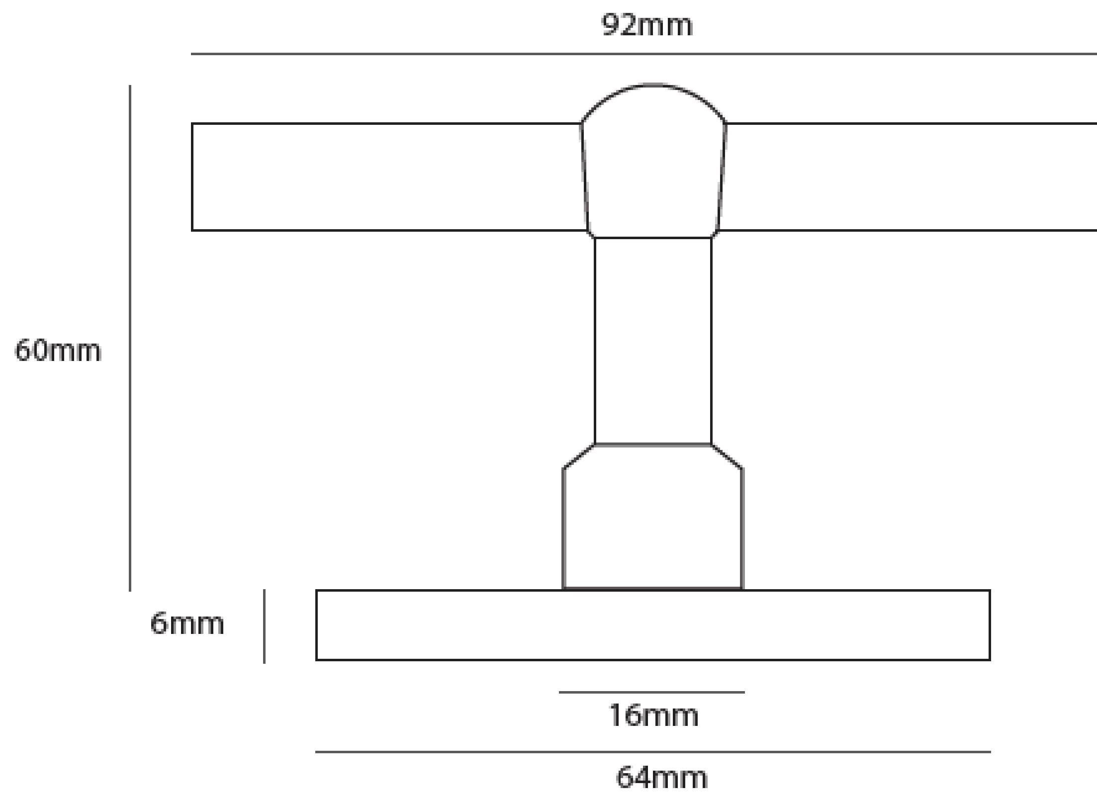
Side view
