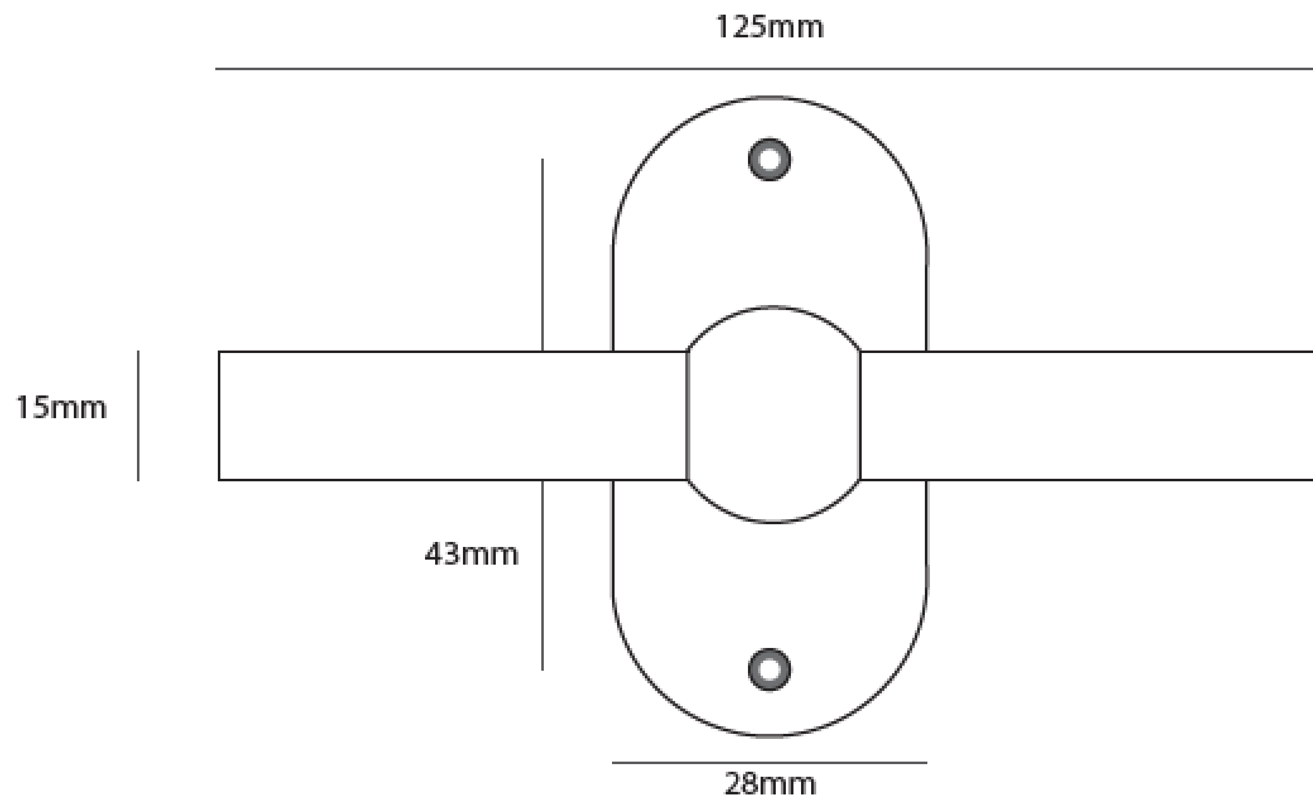
Top view
